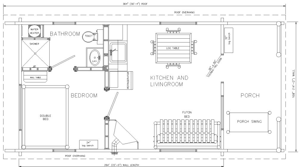
14x22 FLOOR PLAN
